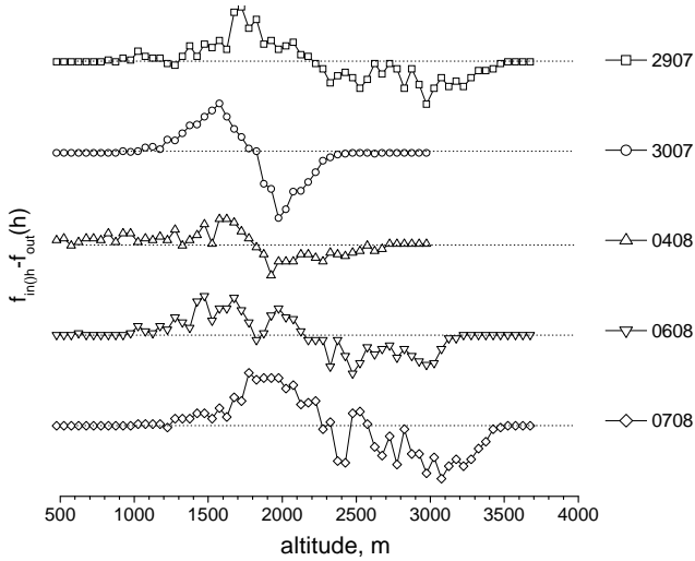
Figure 8 Distributions of thermal entering and exiting altitudes f_{in}(h) - f_{out}(h) for JWGC7.
