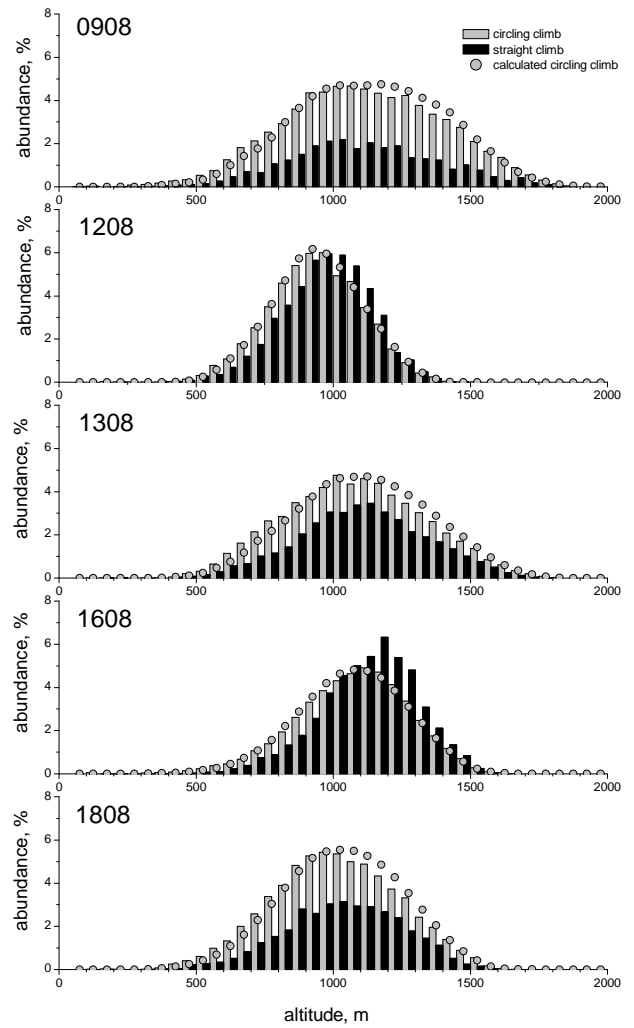
Figure 9 Circling climb altitude distributions f_c^c(h) (grey columns) and straight flight climb altitude distribution f_c^s(h) (black columns) for EGC7. Grey circles represent and circling climb altitude distributions calculated from thermal entering and exiting distributions.
