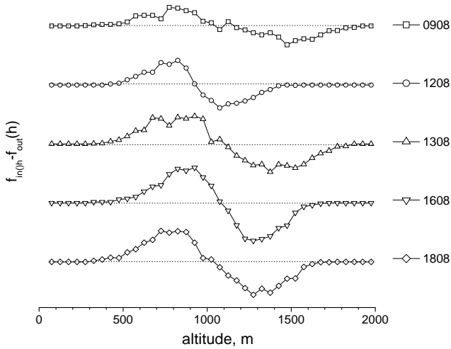
Figure 7 Distributions of thermal entering and exiting altitudes f_{in}(h) - f_{out}(h) for EGC7.
